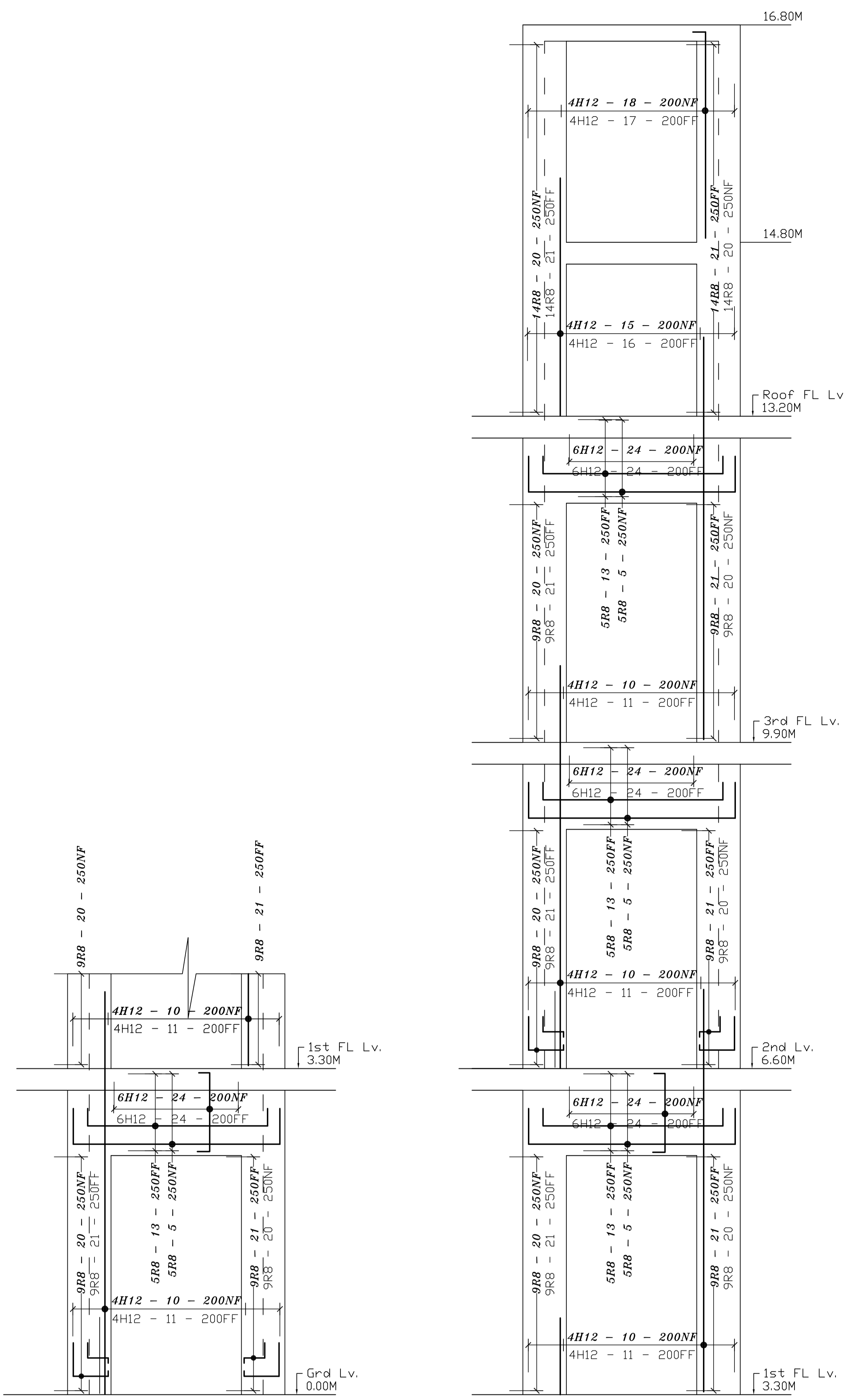
SECT. 3 - 3
